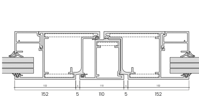
► BLINDALL 60 - NODO CENTRALE BLINDALL 60 - MULLION JOINT
