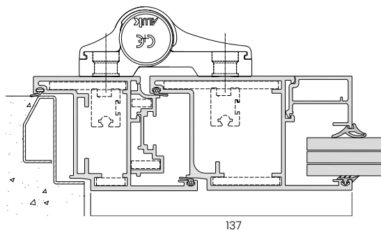
► BLINDALL 60 - NODO LATERALE BLINDALL 60 - LATERAL JOINT
